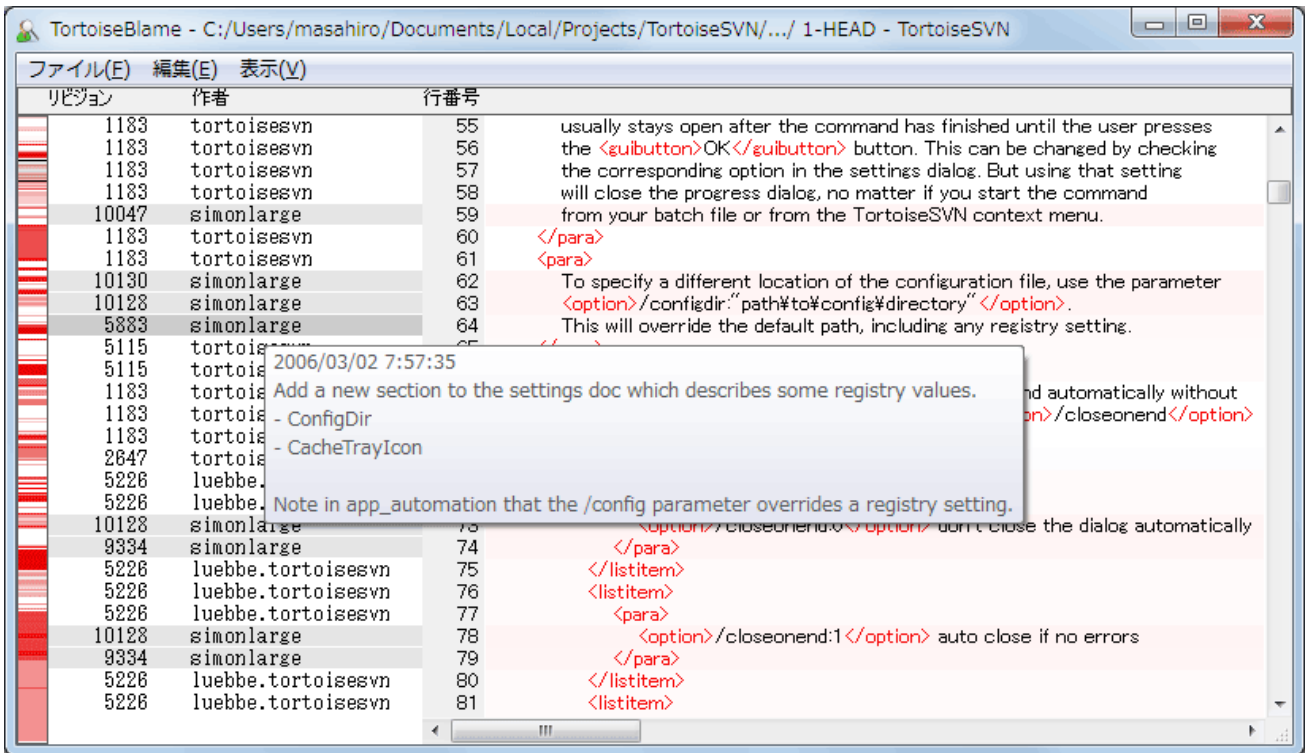
図4.61 TortoiseBlame
