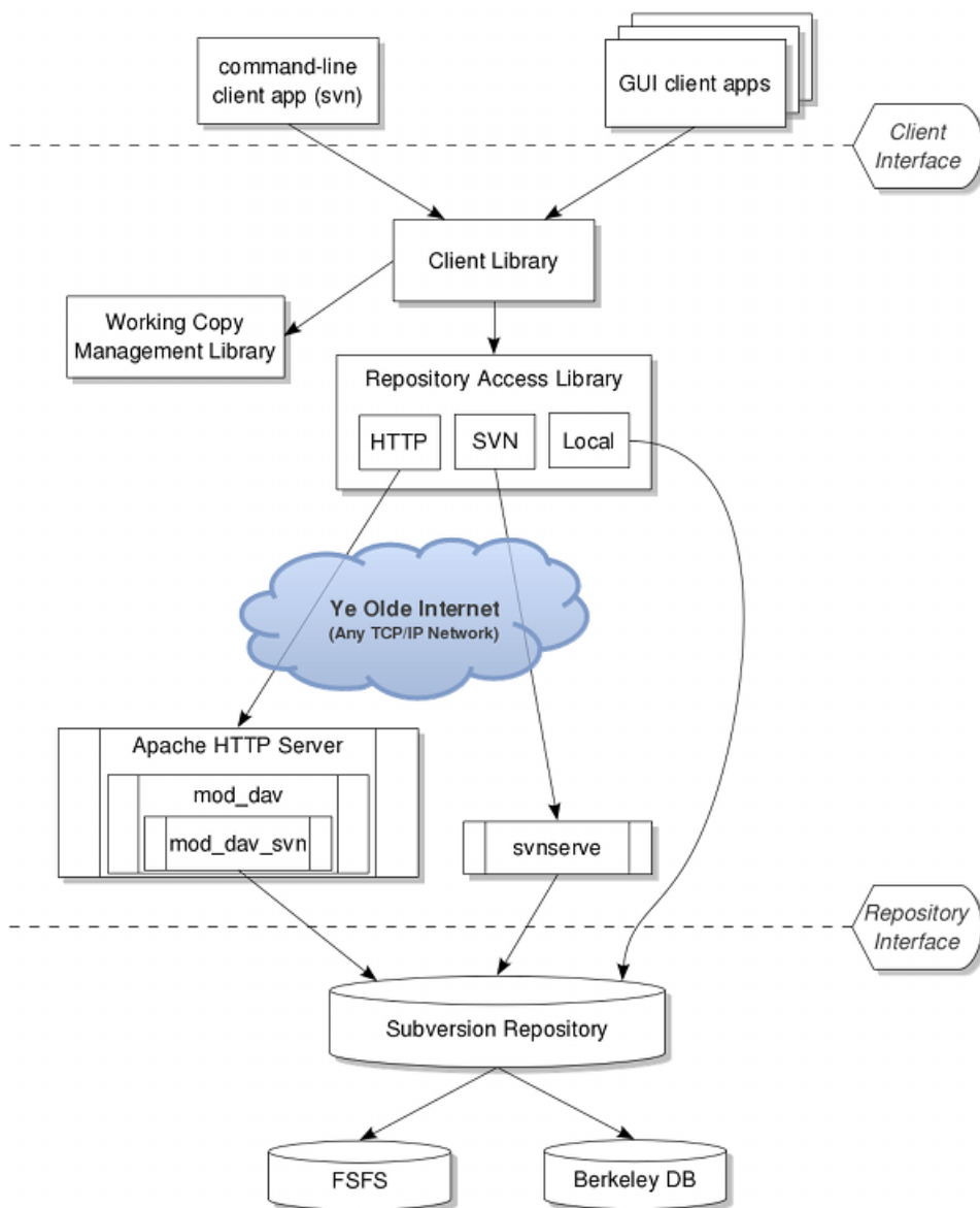
Figure 1. Subversion's architecture
