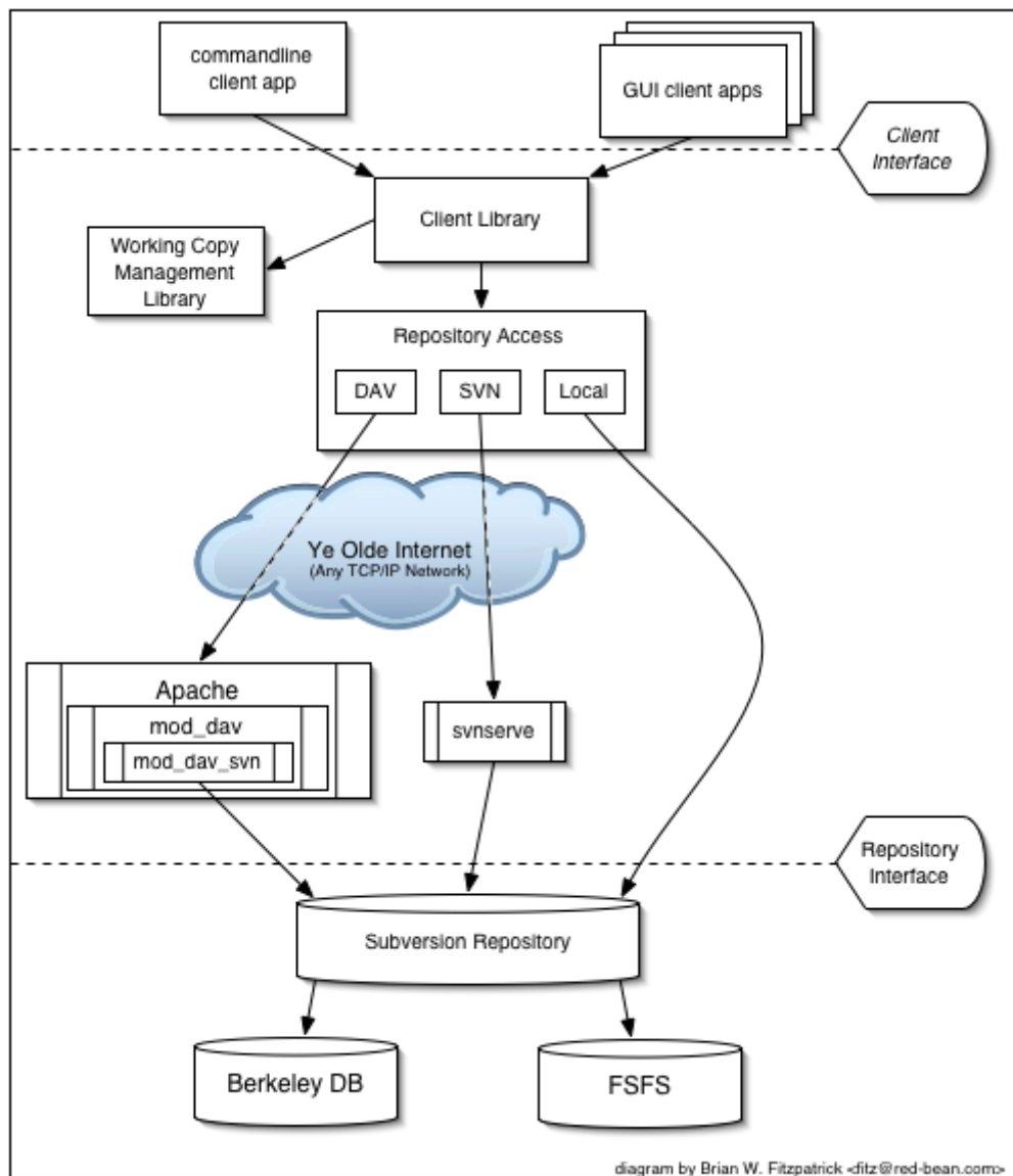
Figure 1. Subversion's architecture
